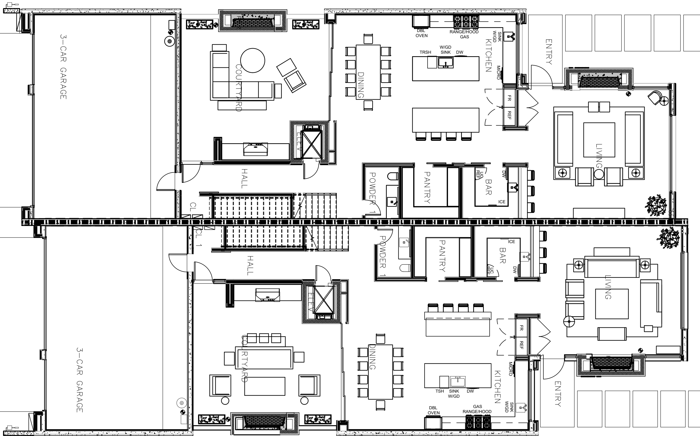
1 I-FP.1 OVERALL MAIN LEVEL FURNITURE PLAN SCALE 1/8"=1'-0"
